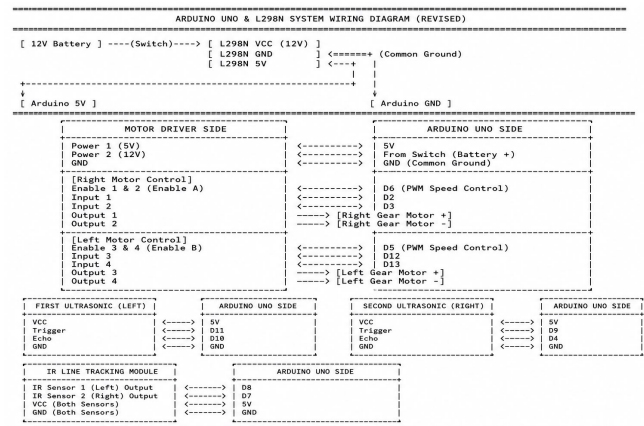
Fig. 6. Autonomous Vehicle Wiring Diagram
