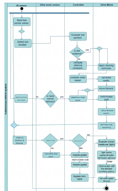
Fig. 3. Activity Diagram
