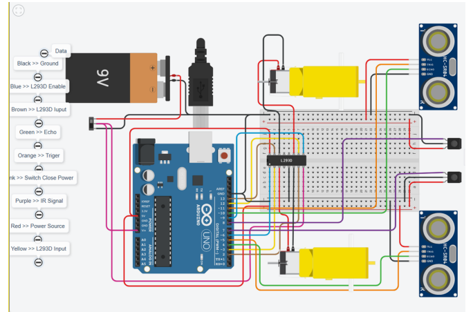
Fig. 9. System Wiring Diagram
